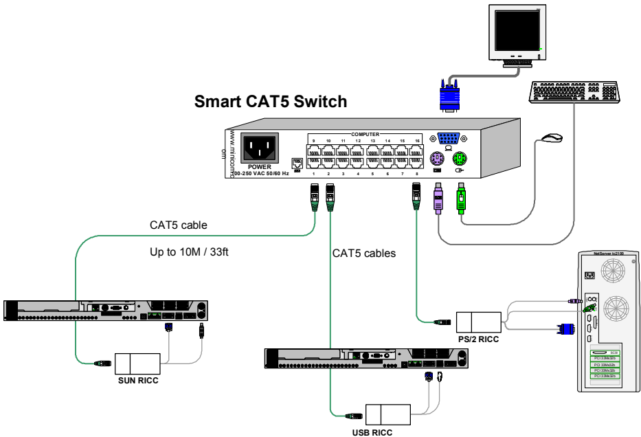
Figure 4 Smart CAT5 system connections
