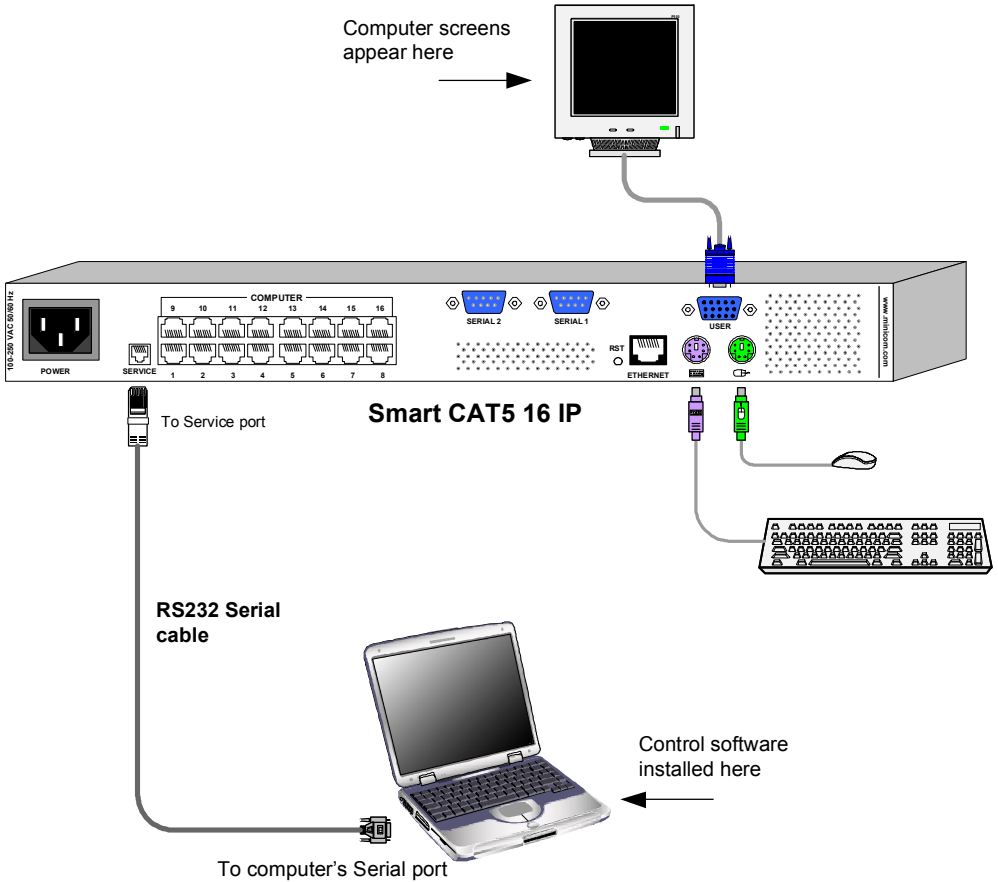
Figure 8 Smart 16 IP with RS232 Serial cable
